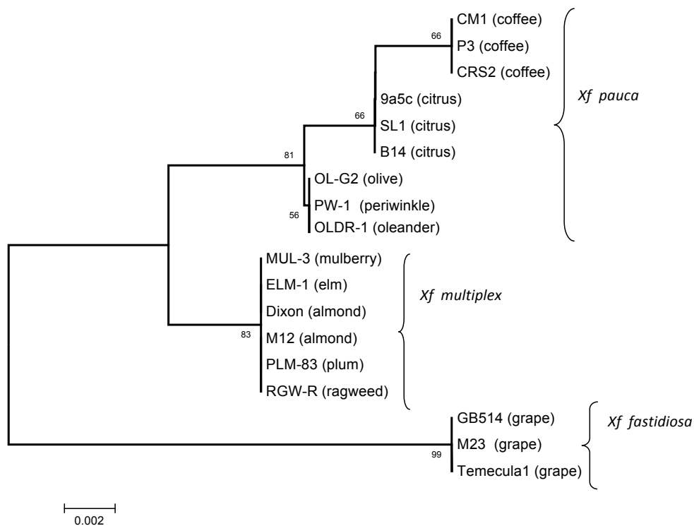
Fig. 3. Phylogenetic trees generated by the Neighbor-Joining method from the alignment of the partial nucleotide sequence of the DNA gyrase subunit B (gyrB) gene using MEGA (Version 5). Bootstrap values for 1000 replicates are shown at the main branches. Branch length is proportional to the number of nucleotide changes. Accession Nos. of GenBank sequences are: AF534974 (CM1); AF534972 (P3); AF534970 (CRS2); AE003849 (9a5c); AF534969 (SL1); AF534968 (B14); AF534965 (MUL-3); AF534966 (ELM-1); EU026153 (Dixon); CP000941 (M12); AF534962 (PLM-83); AF534963 (RGW-R); CP002165 (GB514); CP001011 (M23); AE009442 (Temecula). Sequences from olive, periwinkle and oleander were deposited under the following accession Nos.: KJ406212 (OL-G2); KJ406260 (PW-1); KJ406261 (OLDR-1).
